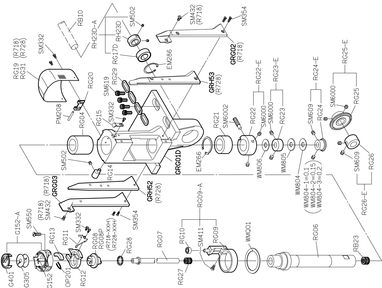
PARTS LIST FOR RG GROUP
