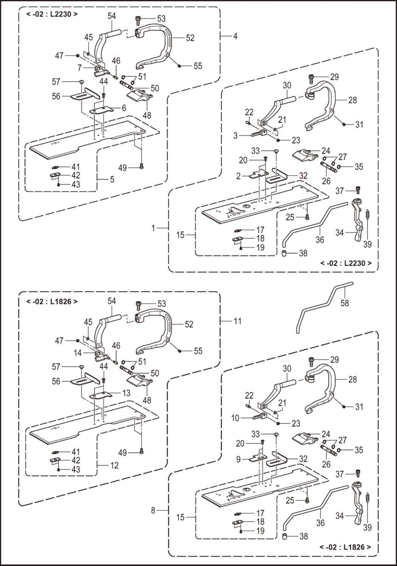
F3 . 压脚装置 / Presser foot mechanism
