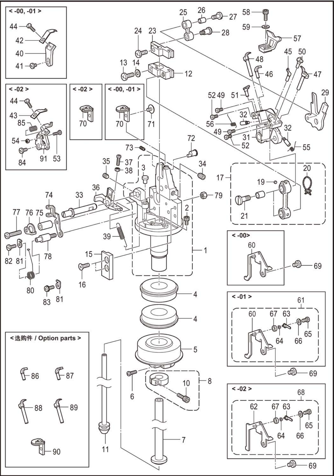
L. 双链式弯针装置 / Double chain stitch looper mechanism
