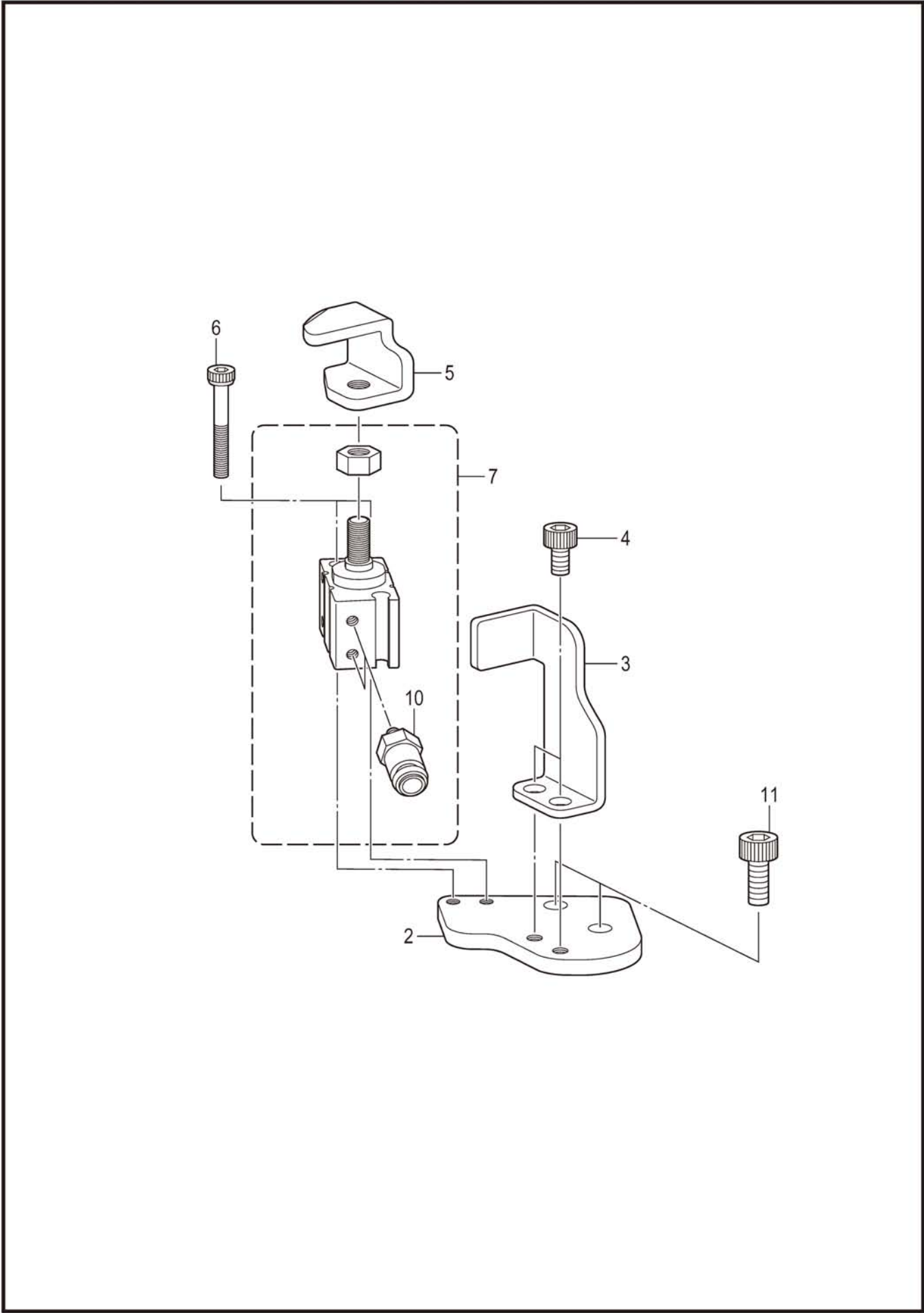
R . 面线剪切装置 / Upper thread trimmer mechanism
