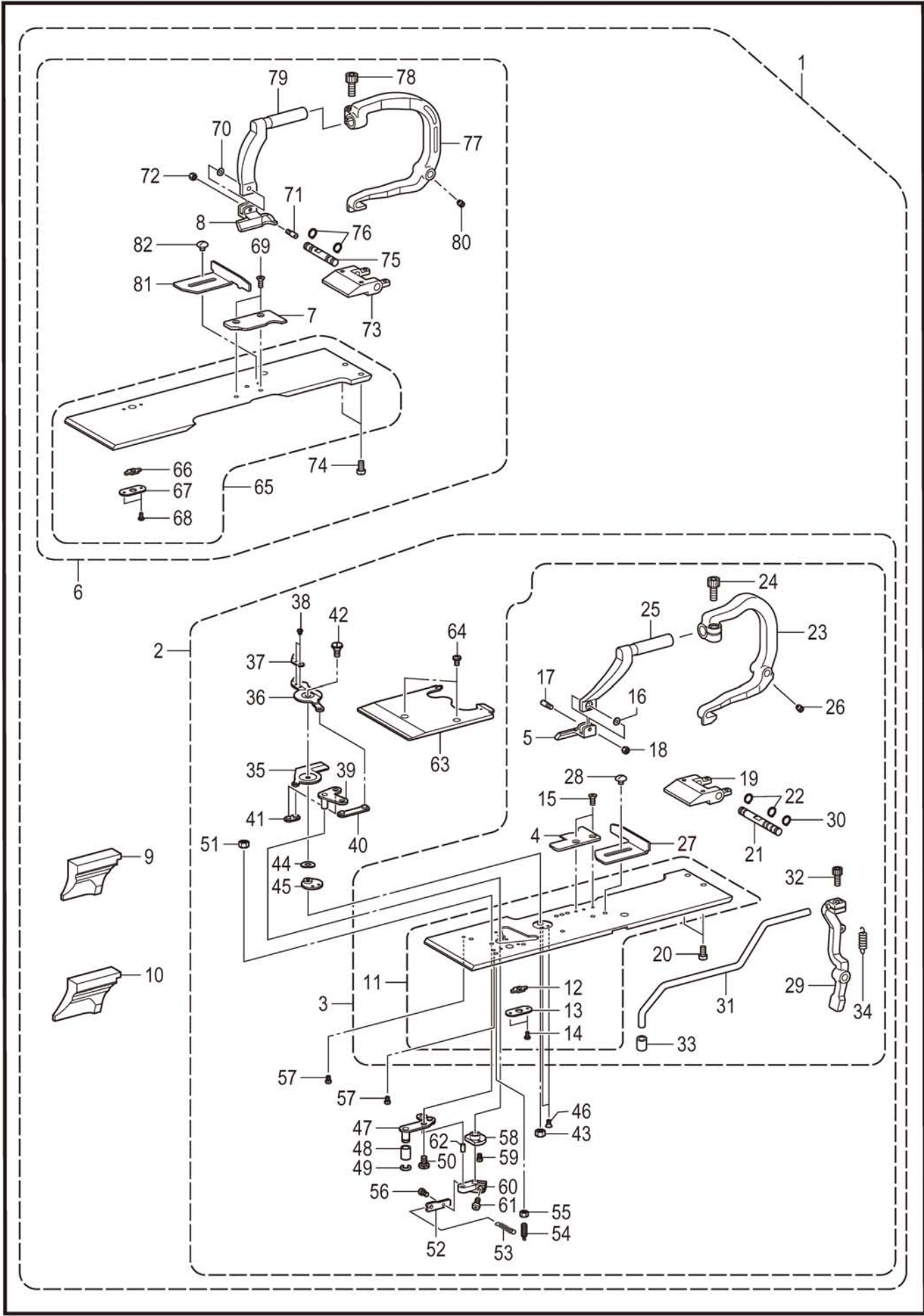
AA1. 附属装置 / Attachment set
