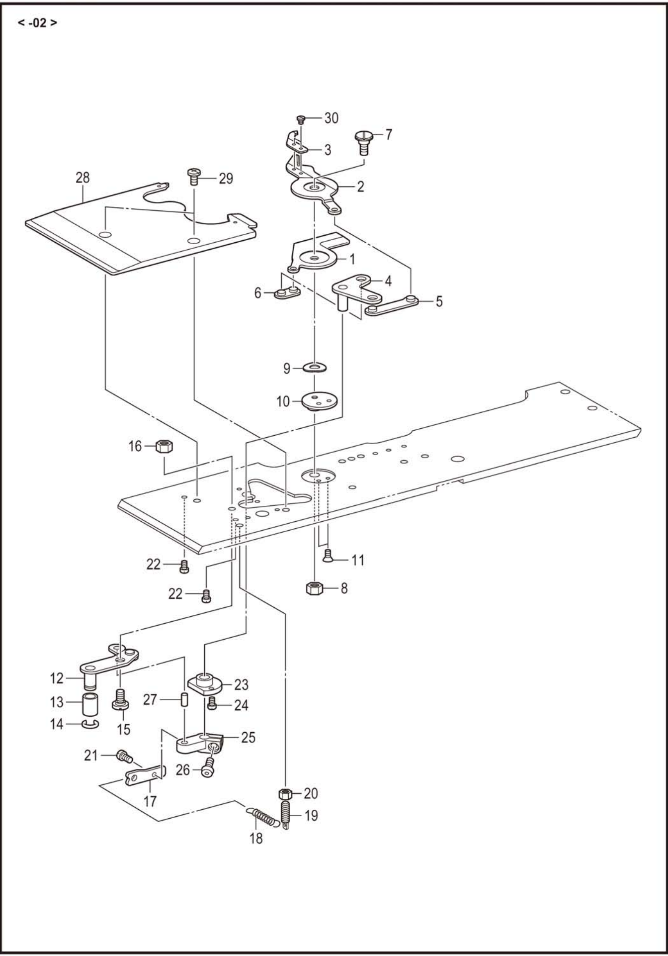
Q2 . 切线装置 / Thread trimmer mechanism
