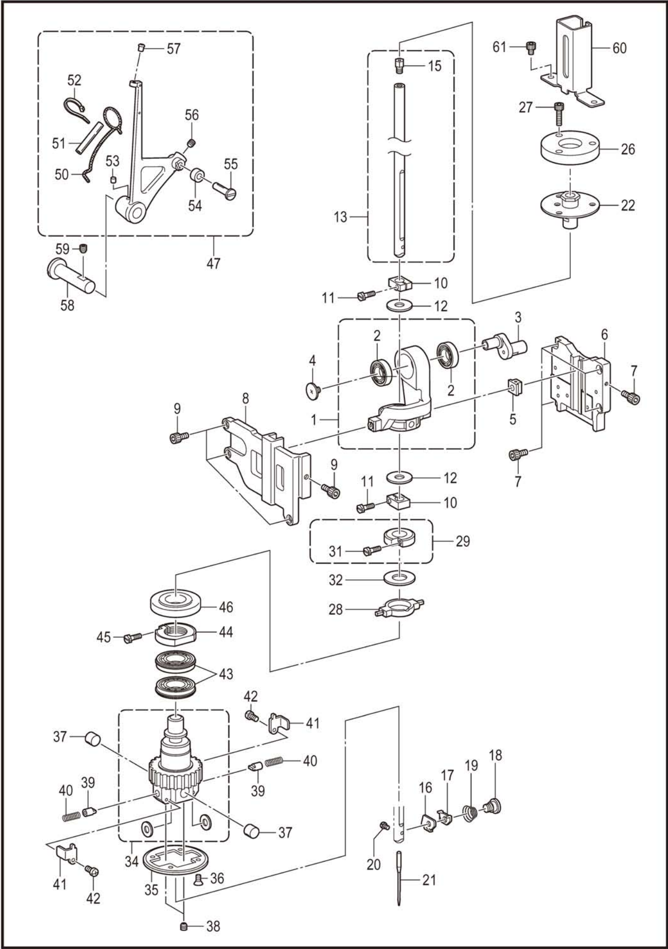
B. 针杆·挑线杆装置 / Needle bar and thread take-up mechanism
