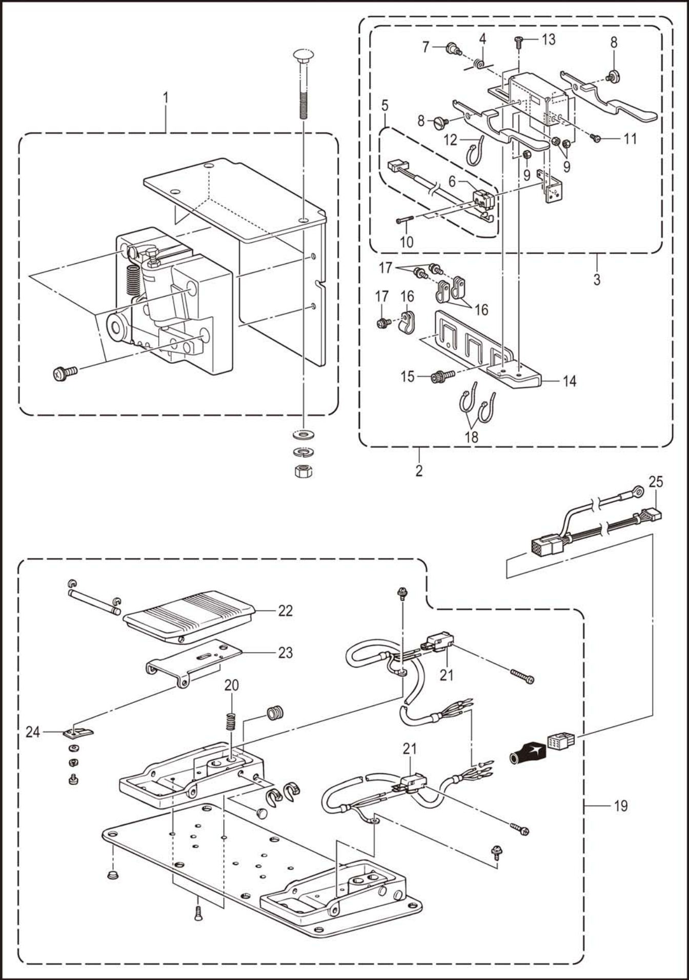
Y. 踏板开关关系 / Foot switch pedal mechanism
