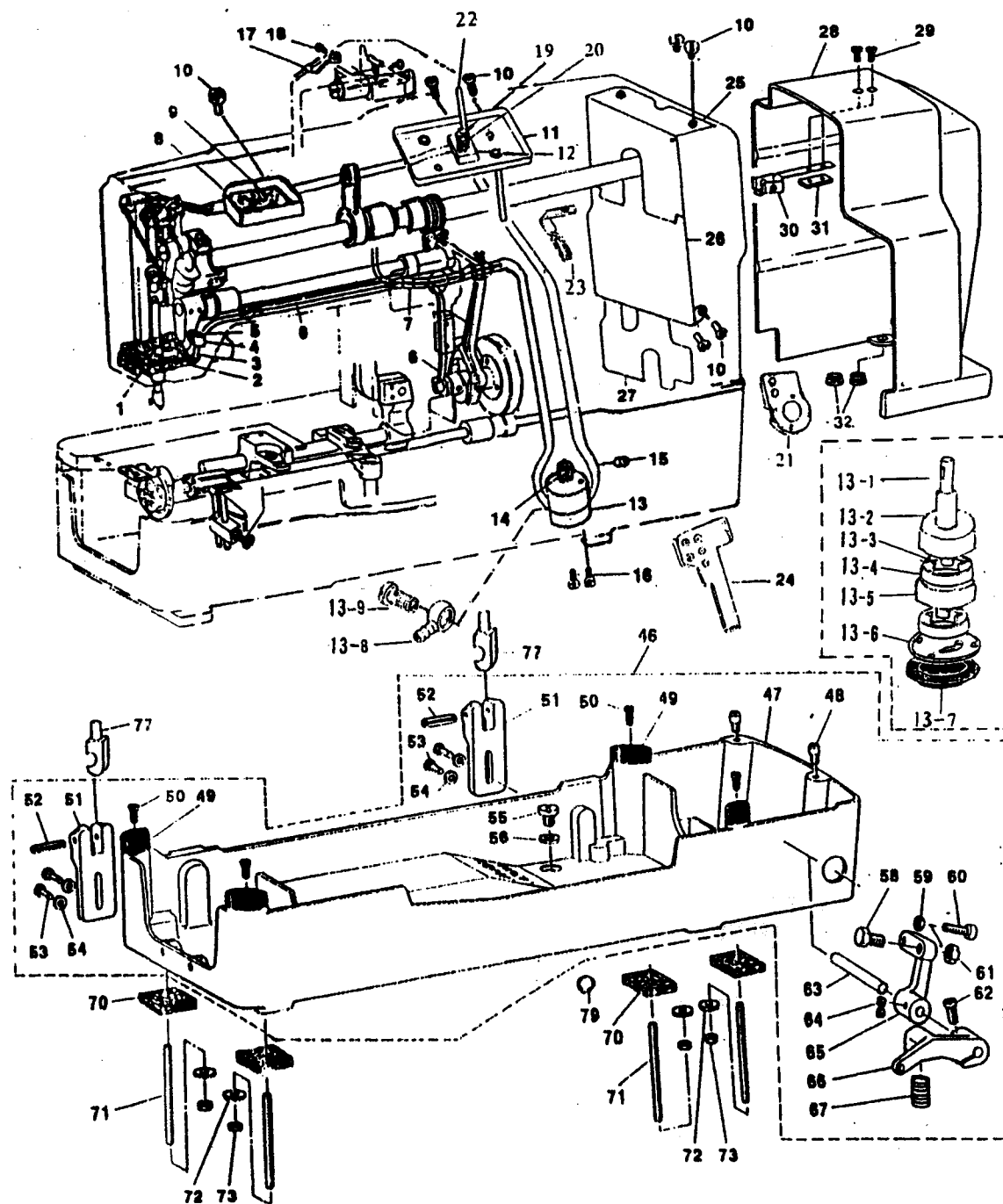
CYLINDER BED MACHINE OIL RESERVOIR
