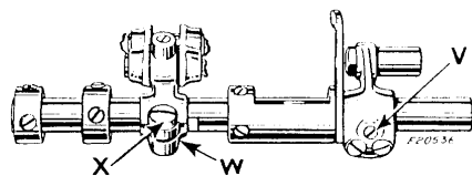
Fig. 29. Feed Lift Crank and Link Assembly
