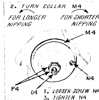
Fig. 56. Adjustments on Automatic Thread Nipper
