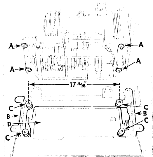
Fig. 5. Setting Up the Machine
