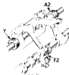
Fig. 31. Feed Rocker and Feed Bar Assembly
