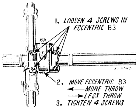
Fig. 46. Showing Spreader Driving Eccentric Screws
