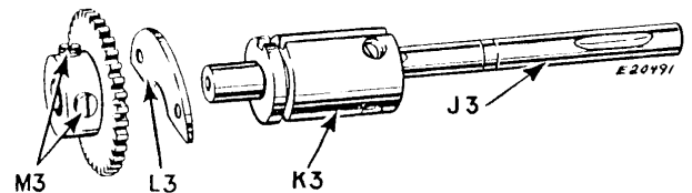
Fig. 50. Looper Carrier Assembly
