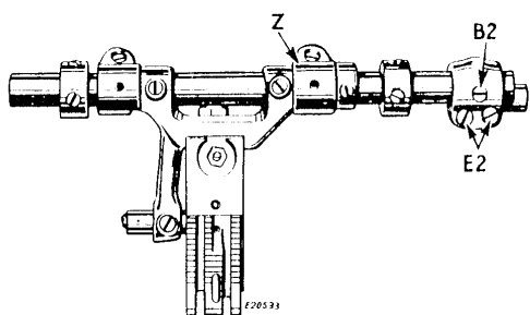
Fig. 33. Feed Driving Rock Shaft Crank and Feed Rocker Assembly
