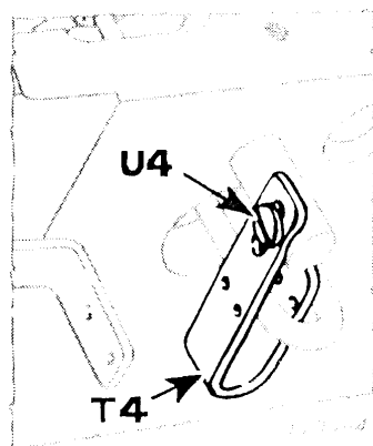
Fig. 58. Adjustment of Looper Thread Take-up
