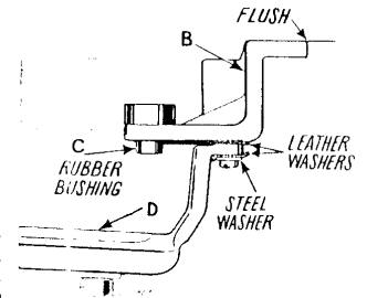
Fig. 4. Hanger and Oil Pan Assembled
