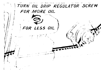
Fig. 66. Adjustment on Thread Oiler
