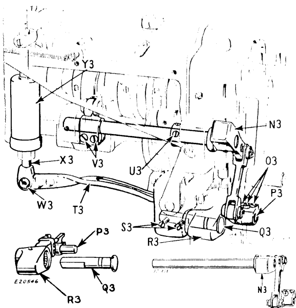
Fig. 51. To Remove Alternating Presser Mechanism
