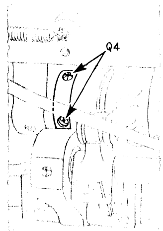
Fig. 55. Automatic Thread Nipper Eccentric at Back of Machine
