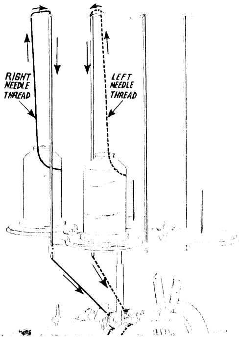
Fig. 16. Needle Threading
