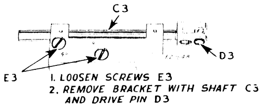
Fig. 48. Spreader Shaft and Bracket
