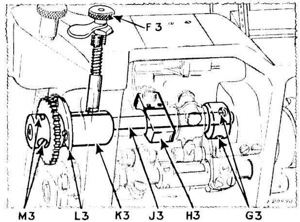
Fig. 49. To Remove Looper Carrier Assembly
