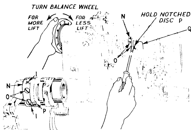
Fig. 26. Regulating Lift of Pressers
