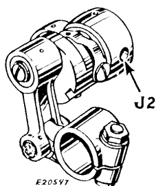
Fig. 37. Feed Lift Eccentric
