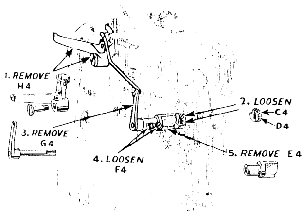
Fig. 53. To Remove Presser Lifting Mechanism
