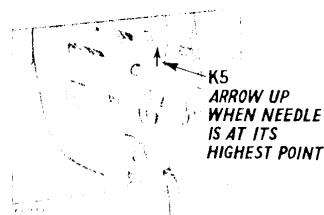
Fig. 64. Showing Timing Arrow on Bed Shaft Pulley
