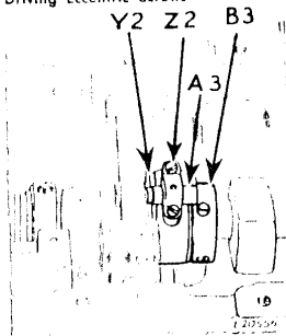
Fig. 47. Sidewise Adjustment of Spreader
