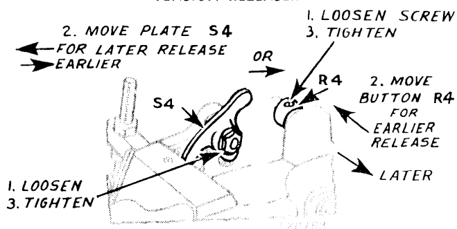
Fig. 57. Adjustments on Needle Thread Tension Releaser
