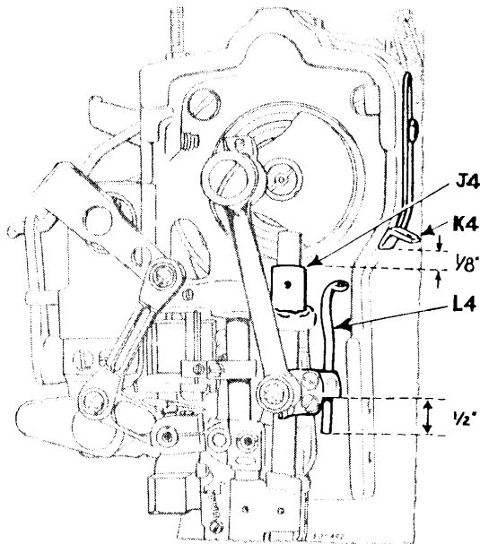
Fig. 54. Adjustment of Needle Thread Take-up and Loop Setting Eyelet
