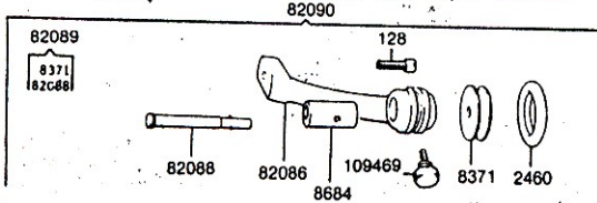
BOBBIN WINDER COMPLETE FOR M/c. 29K72
