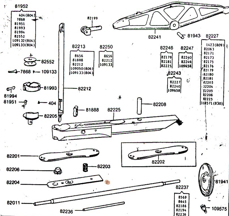
BOBBIN WINDER COMPLETE FOR M/c. 29K72
