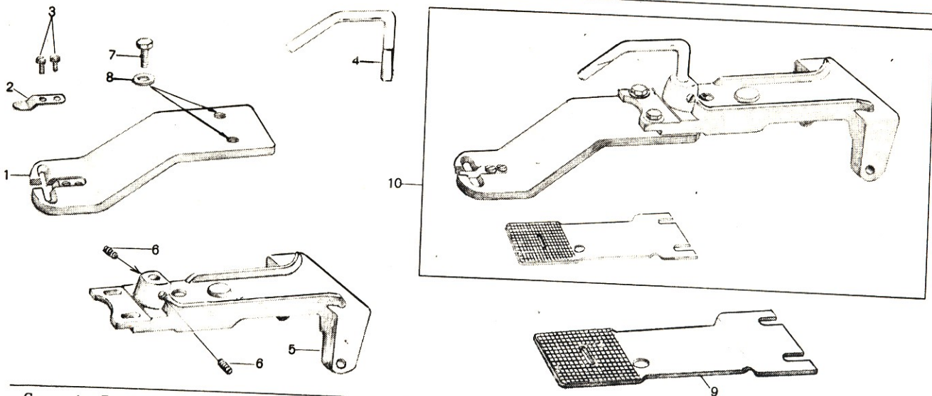
Conversion Parts for 6-12-24 Stitches
