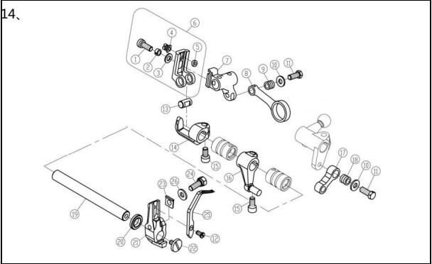
十四、二重环弯针机构(1)/Chainstitch Loper Drive Mechanism(1)
