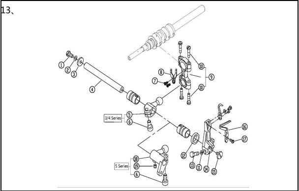
十三、下弯针部件/Lower Loper Drive Mechanism
