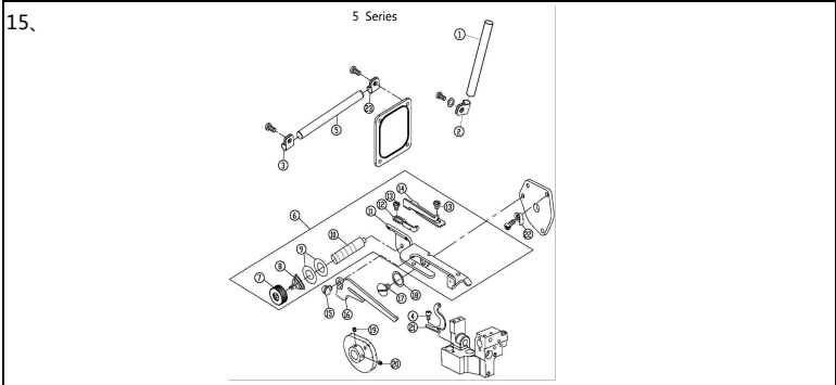
十五、二重环弯针机构(2)/Chainstitch Loper Drive Mechanism(2)
