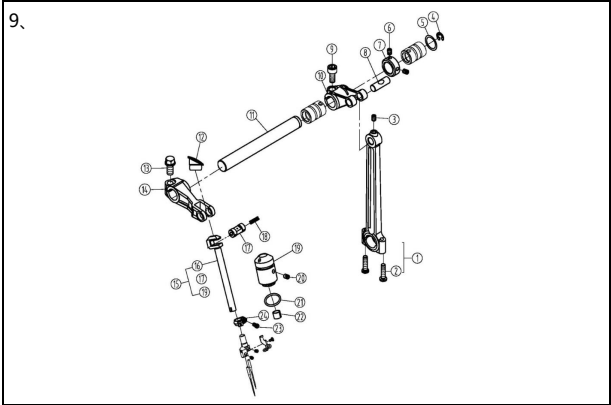
九、针杆部件(1)/Needle Drive Mechanism(1)
