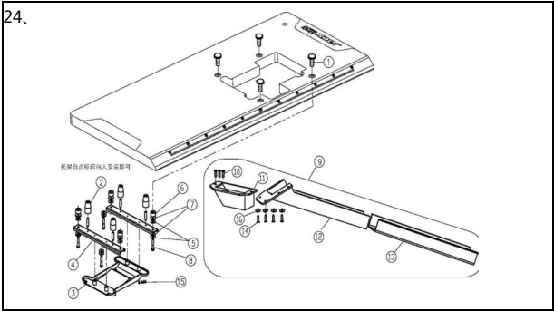
二十四、托盘部件/Part For Semi-Submerged Installation
