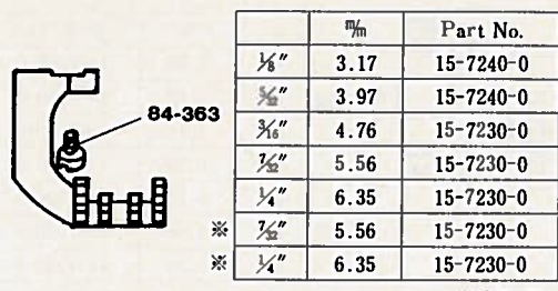
Feed dog (front)
