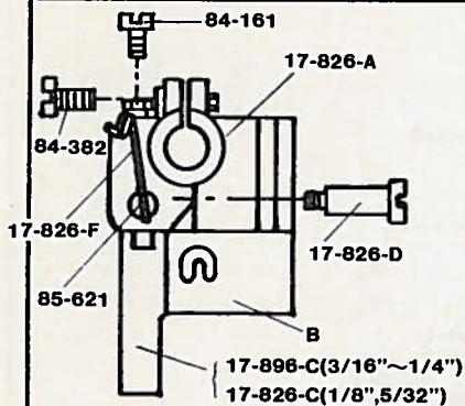
Presser foot (2 Needles)
