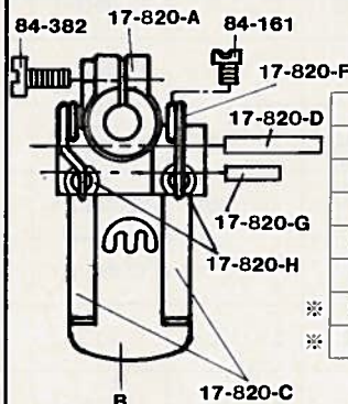
Presser foot (2,3 Needles)
