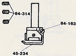
Needle holder (2,3 Needles)
