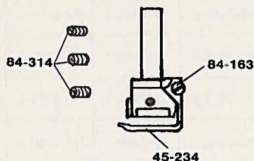
Needle holder (2,3 Needles)
