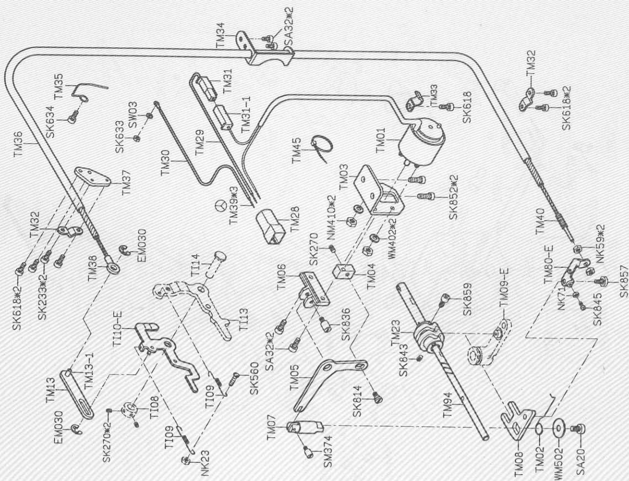
PARTS LIST FOR TM(3) GROUP FOR THREAD TRIMMER
