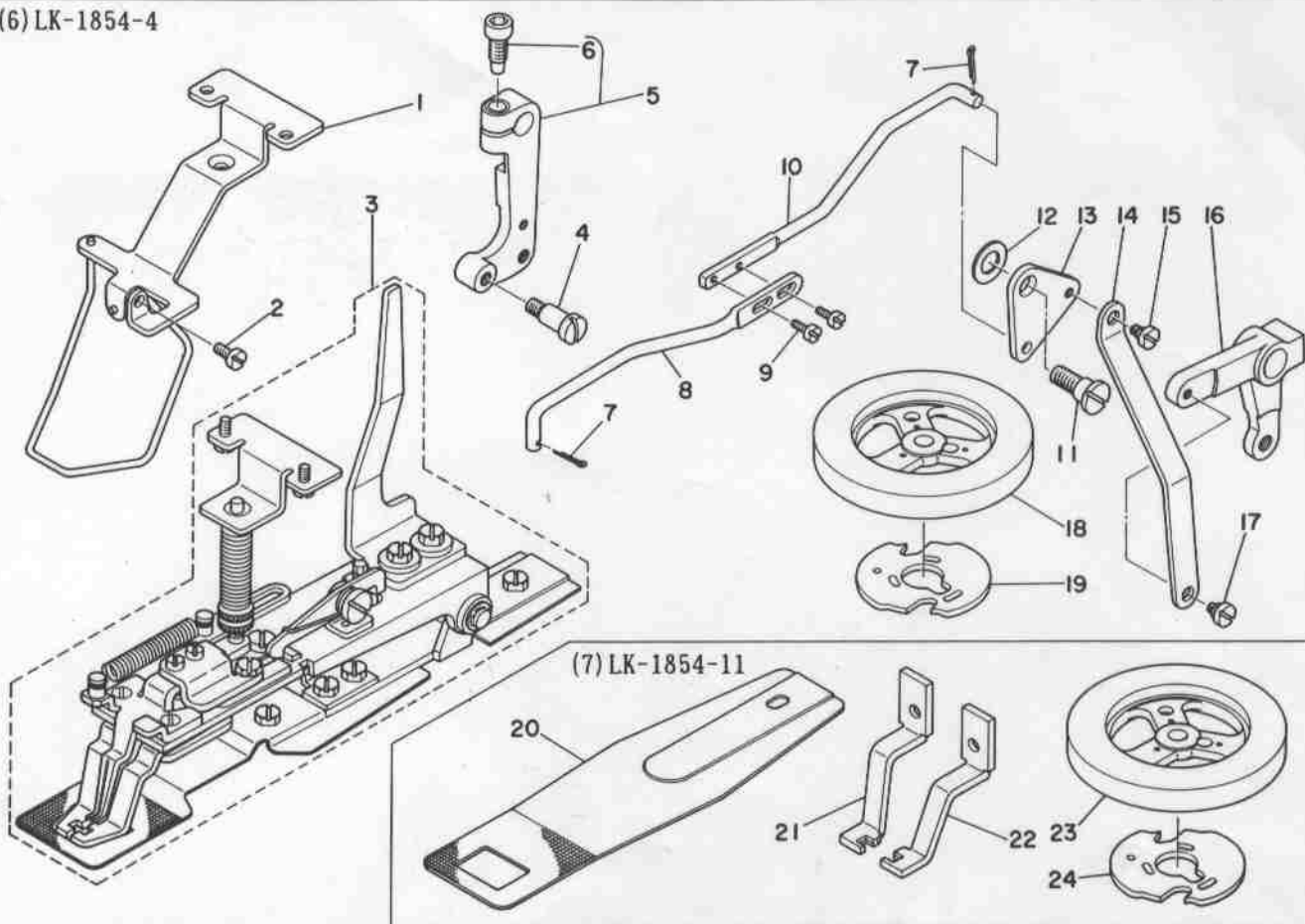
(6) LK-1854-4 TAIL OF EYELET BUTTONHOLE BAR TACKING MACHINE (21 STITCHES) 21針穴門止めミシン
