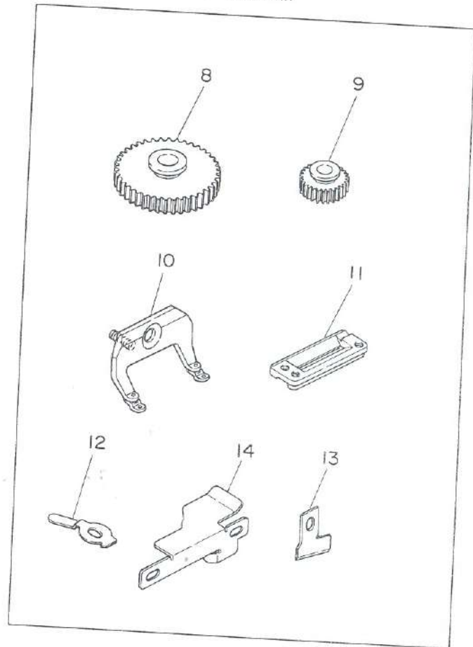
27. EXCLUSIVE PARTS FOR LBH-793S, 793S-1 LBH-793S, 793S-1 専用部品
