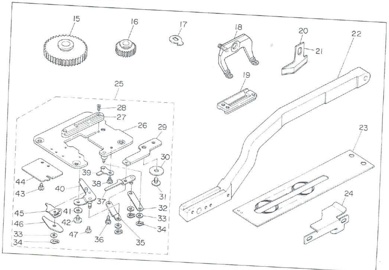
28. EXCLUSIVE PARTS FOR LBH-794S, 794S-1 LBH-794S, 794S-1 専用部品
