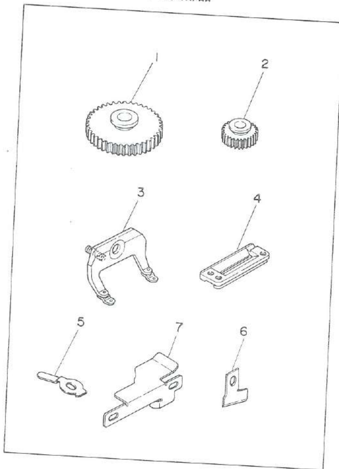
28. EXCLUSIVE PARTS FOR LBH-794S, 794S-1 LBH-794S, 794S-1 専用部品
