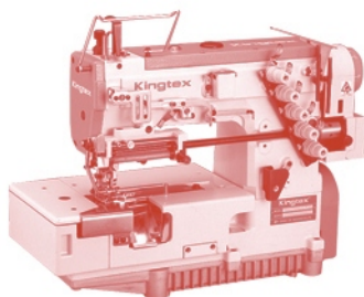
FT6539-0-56M Elastic Tape Or Lace Attaching (With Right Hand Side Fabric Trimmer) 鬆緊帶或蕾絲帶車縫(附右切刀修布裝置)
