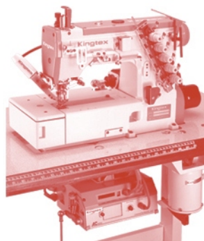
FT6500-0-56M/UFE-1 Electric Under Bed Thread Trimming System For Flat Bed Interlock Machines 電動式自動切線裝置(平台型繡縫機用)
