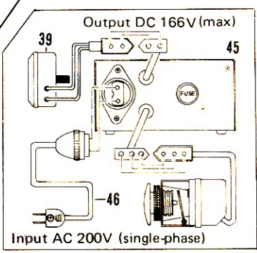
Single-phase wiring diagram (input AC 200V)
