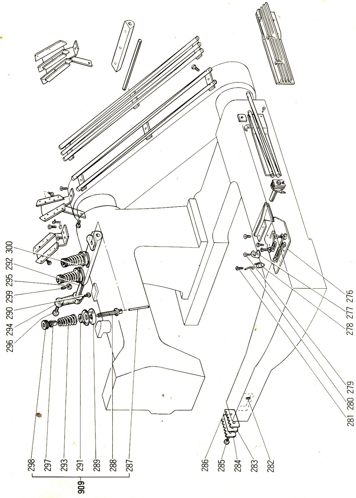
DV440-20--30(DV440·450)形 糸案内、糸調節部分 THREAD GUIDE AND THREAD REGULATING MECHANISM
