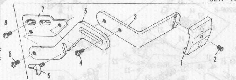
Special Binder Bracket
