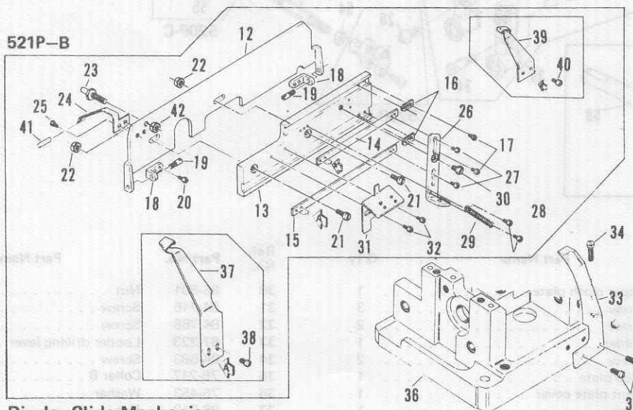
Binder Slide Mechanism
