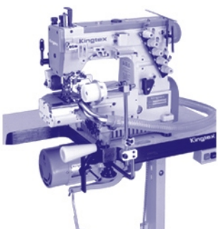
CT6585-0-56M/RP Attaching Pre-Closed Flat Knit Elastic Band Onto Waists Of Tubular Goods. (With Right Knife, Rear Puller & Chips Suction Pipe) 車縫環狀平版寬幅鬆緊帶 (具右切刀修布裝置, 後拖輪及吸屑導管)
