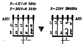
② Netzstecker main connector
